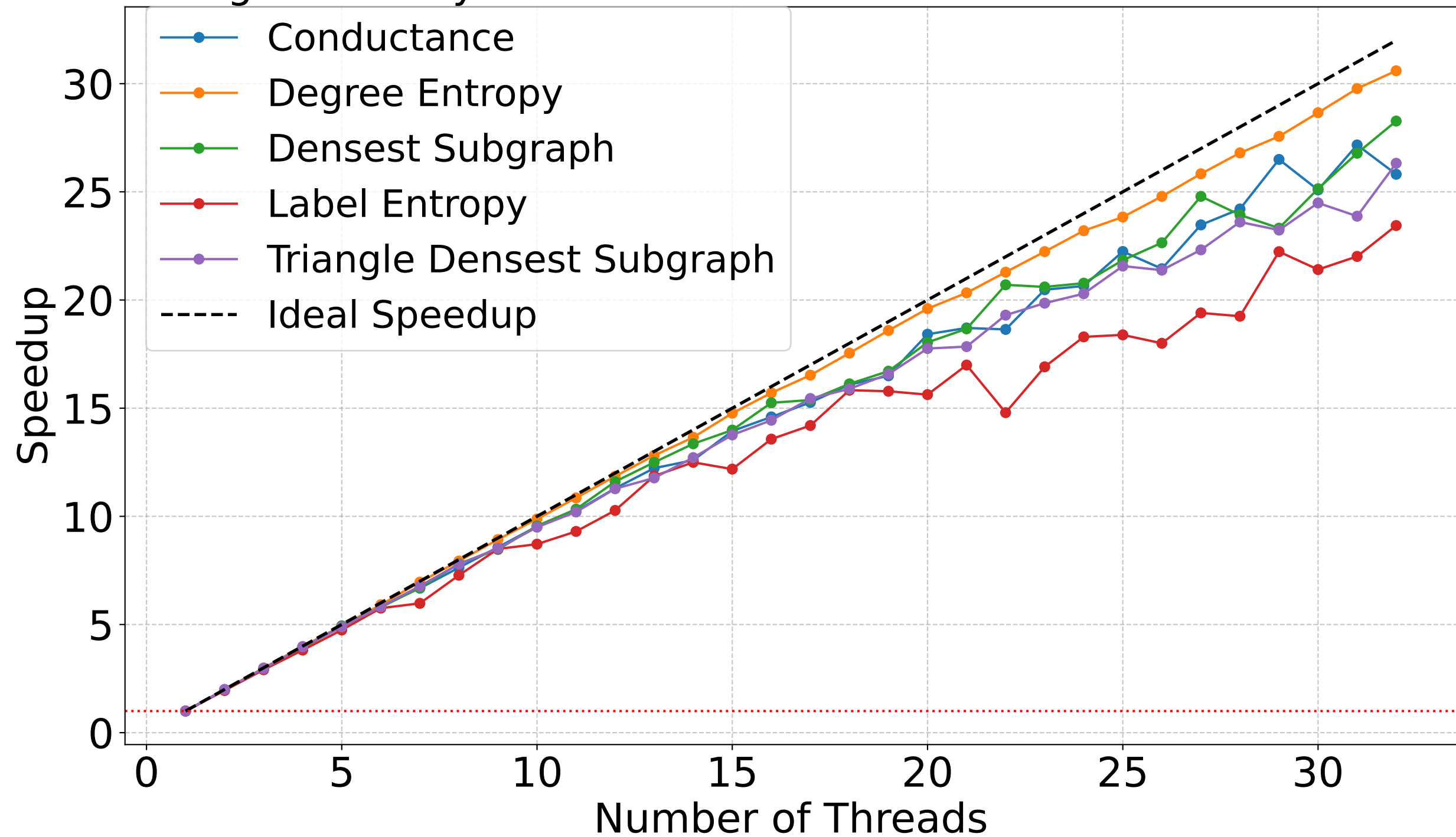
Strong Scalability for Youtube with VNS Run Timeout of 3 seconds
