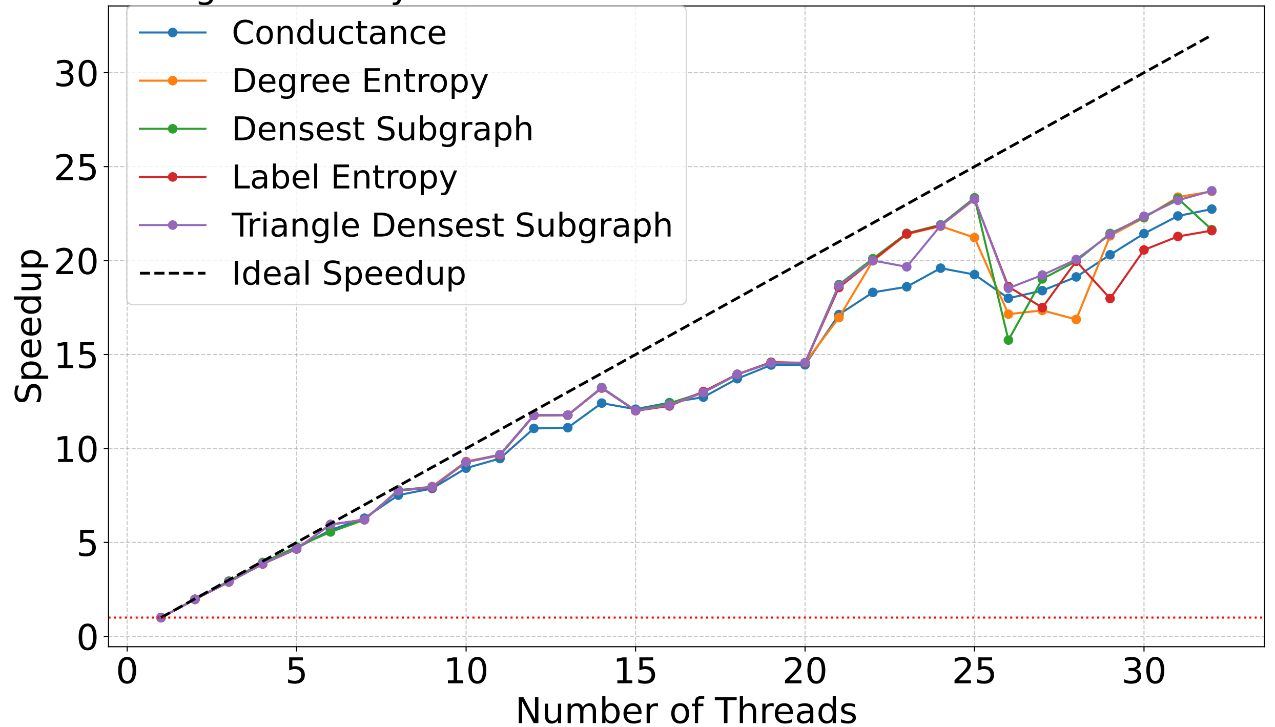
Strong Scalability for Citeseer with VNS Run Timeout of 2 seconds
