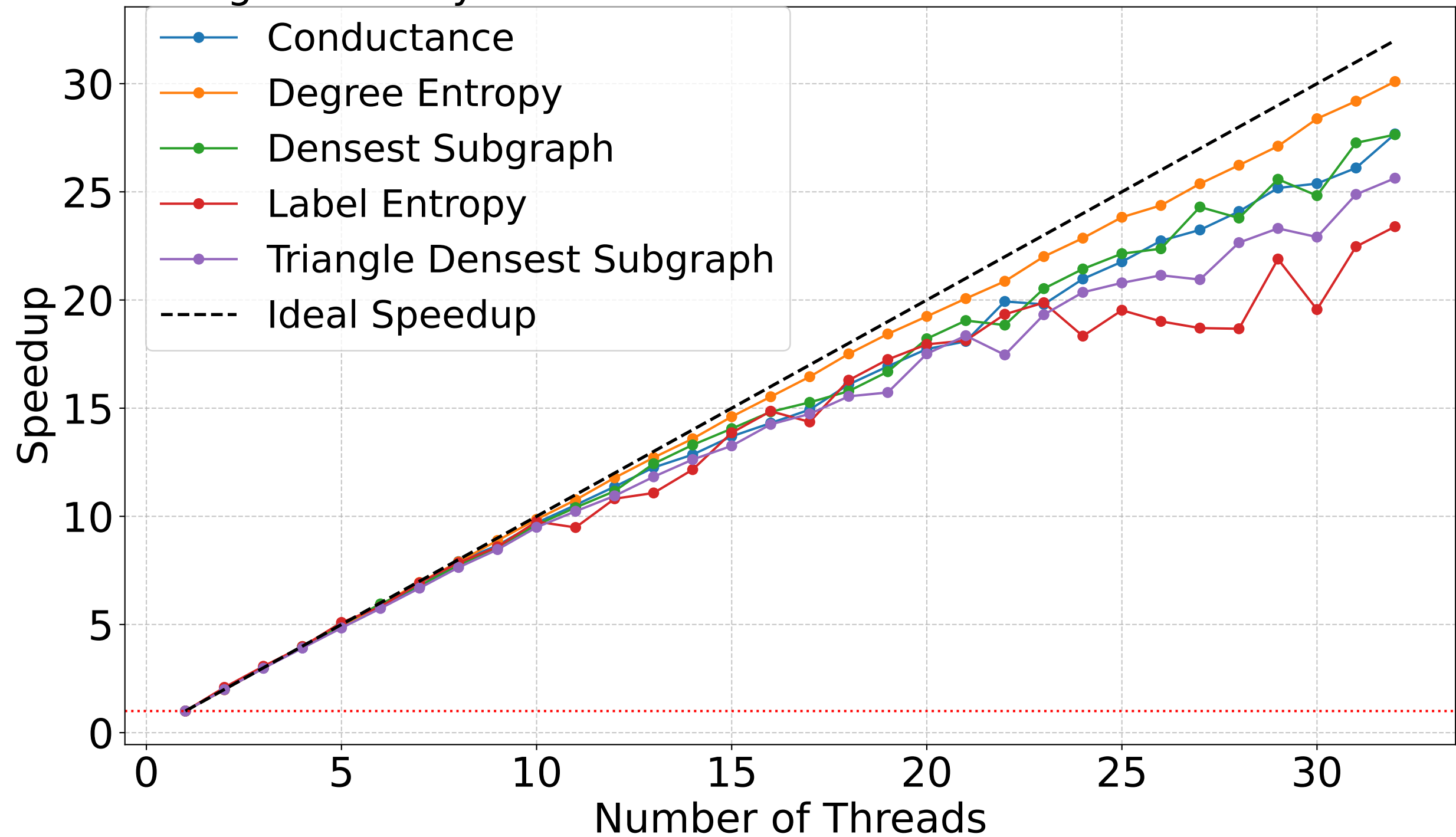
Strong Scalability for Youtube with VNS Run Timeout of 2 seconds
