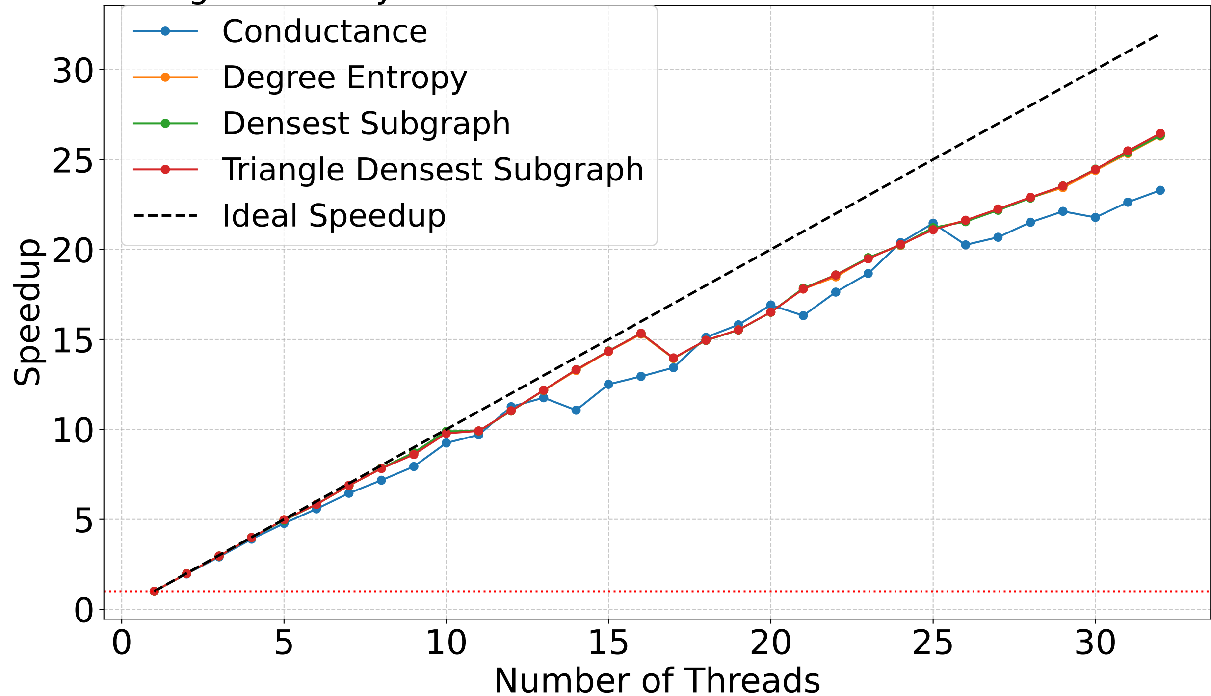
Strong Scalability for Amazon with VNS Run Timeout of 2 seconds
