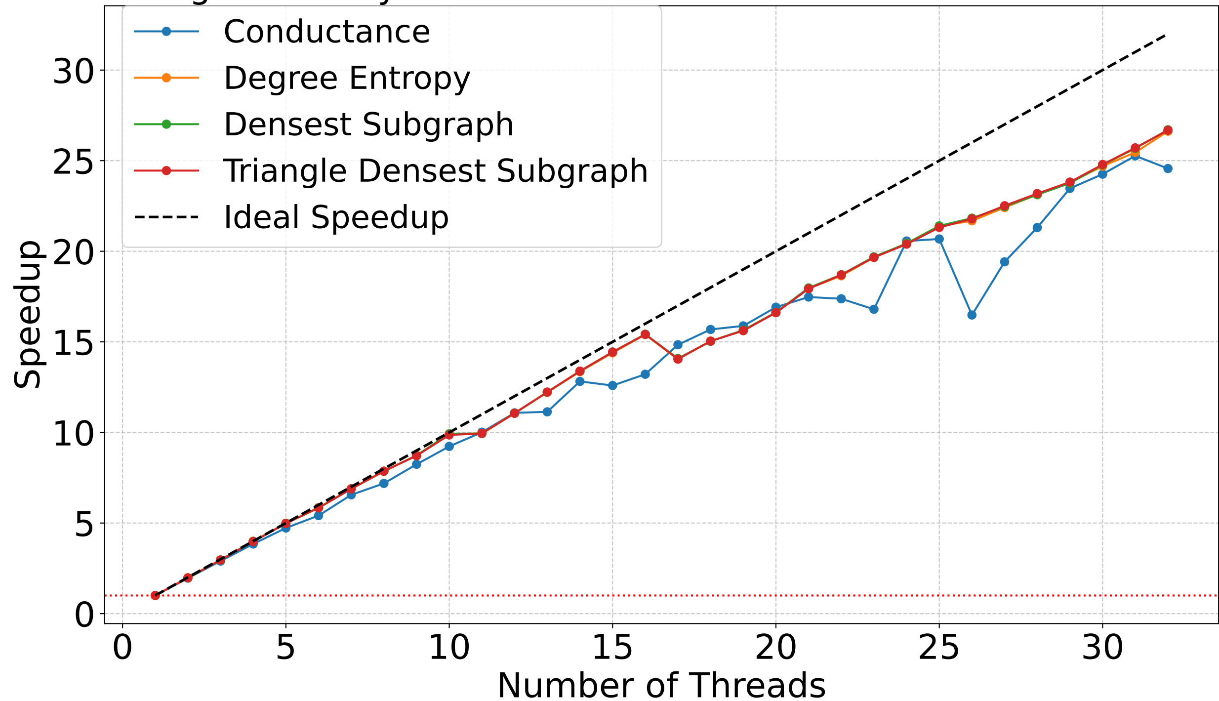
Strong Scalability for Amazon with VNS Run Timeout of 3 seconds
