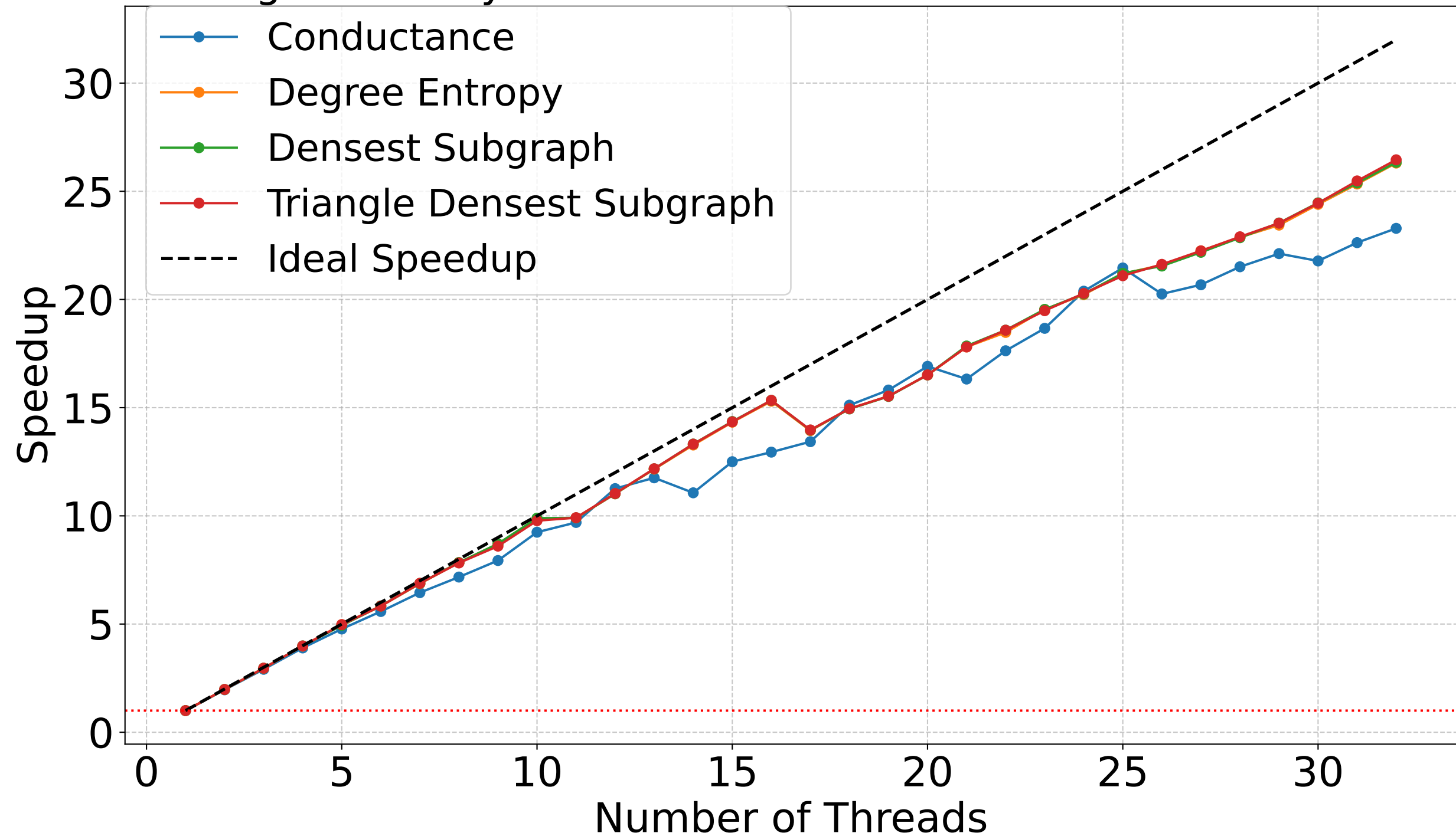
Strong Scalability for DBLP with VNS Run Timeout of 2 seconds
