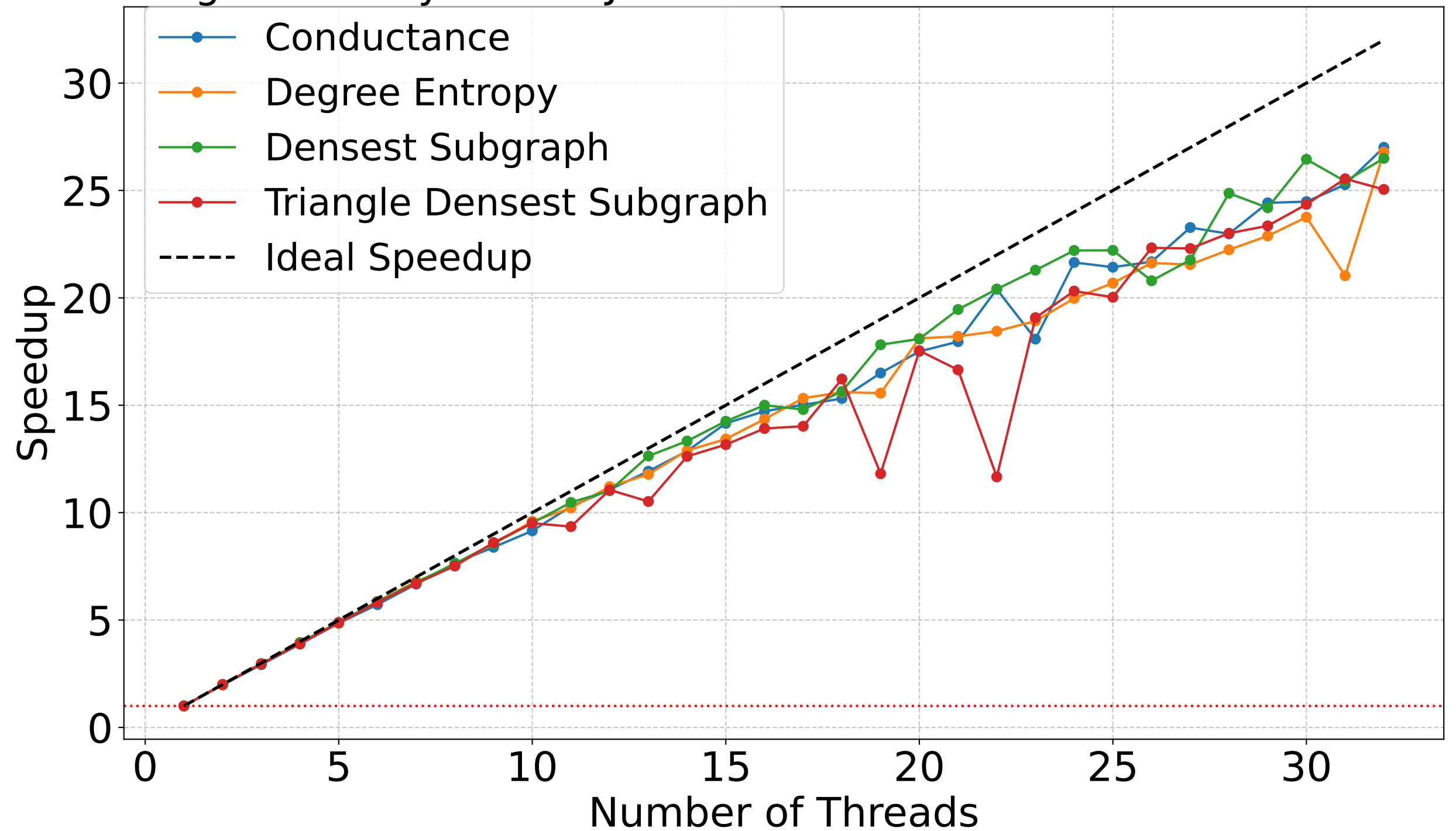
Strong Scalability for LiveJournal with VNS Run Timeout of 2 second
