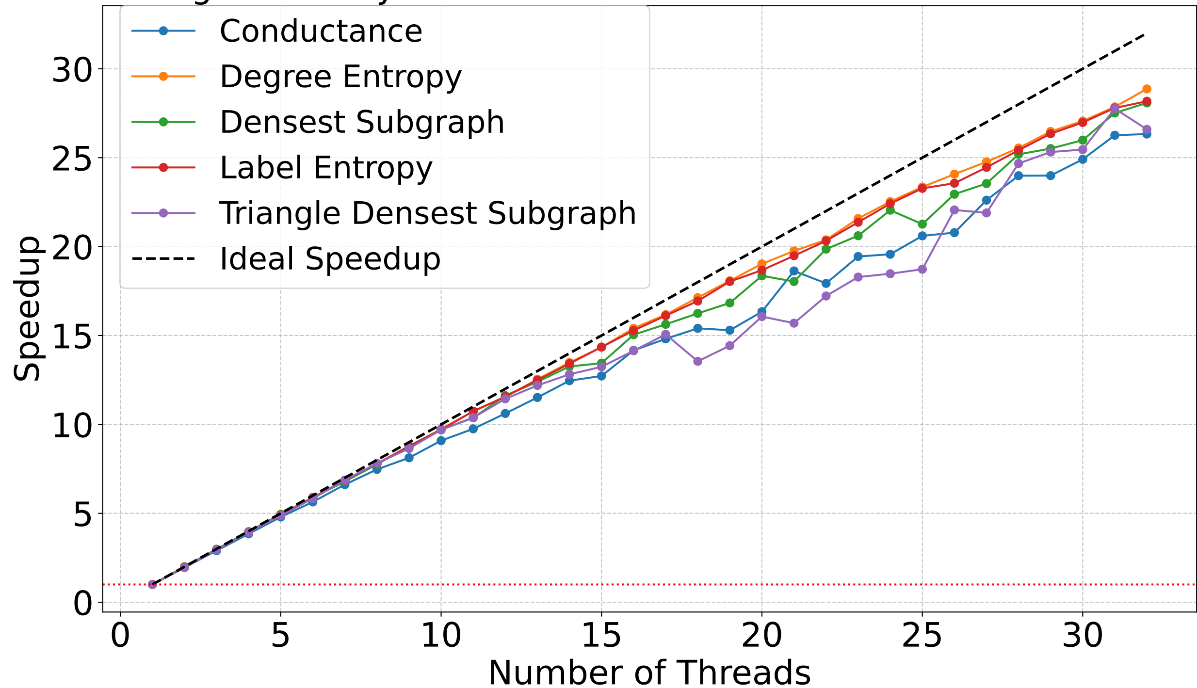
Strong Scalability for Patents with VNS Run Timeout of 1 seconds
