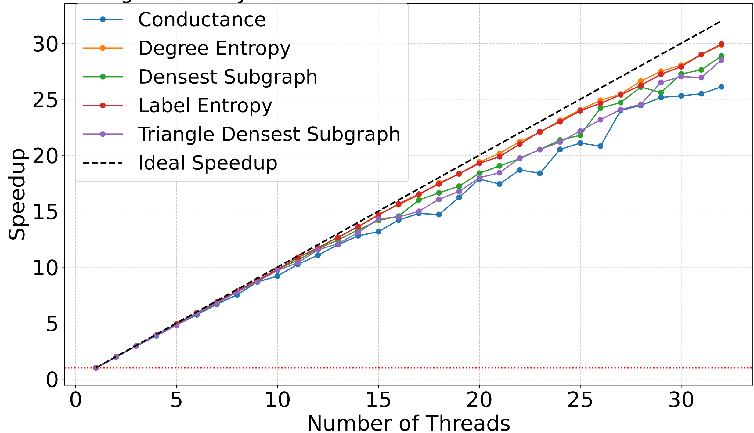
Strong Scalability for Patents with VNS Run Timeout of 2 seconds
