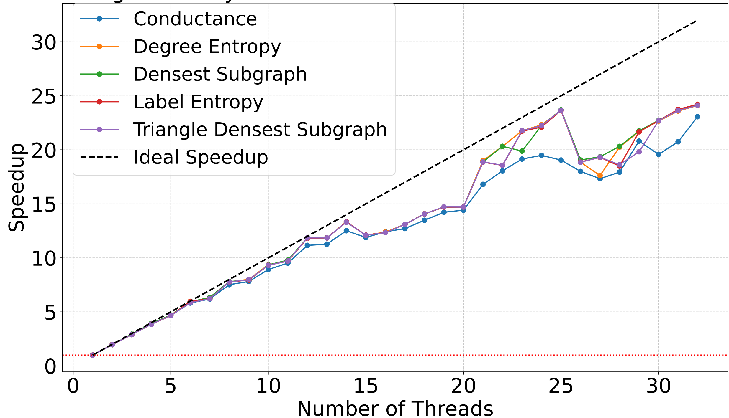
Strong Scalability for Citeseer with VNS Run Timeout of 3 seconds
