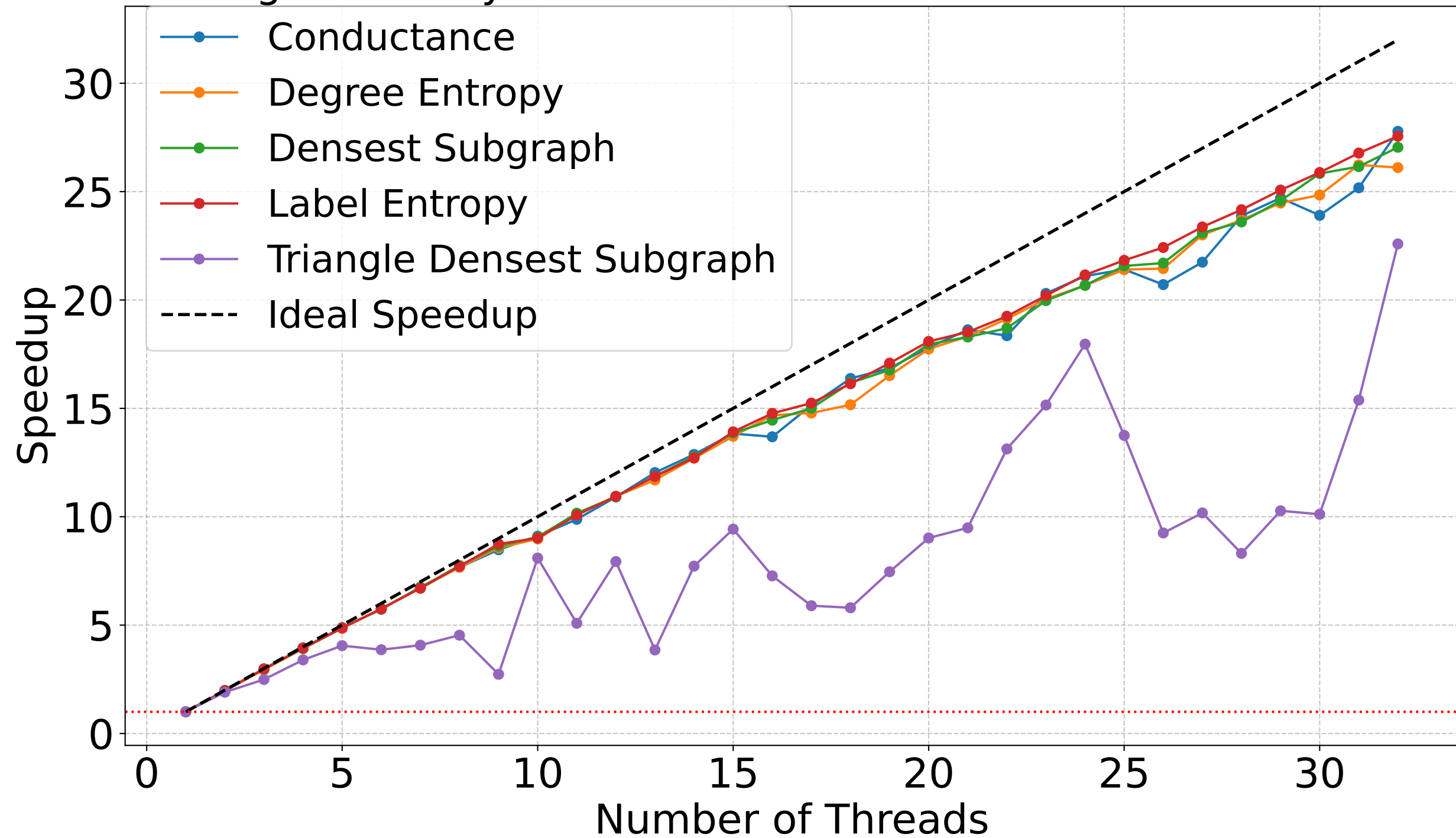
Strong Scalability for DBLP with VNS Run Timeout of 1 seconds
