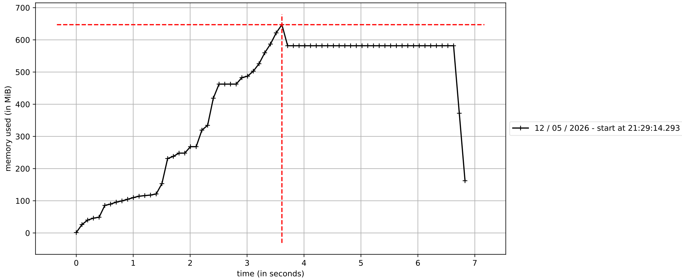
python src/compress/measure_memory_v2.py
