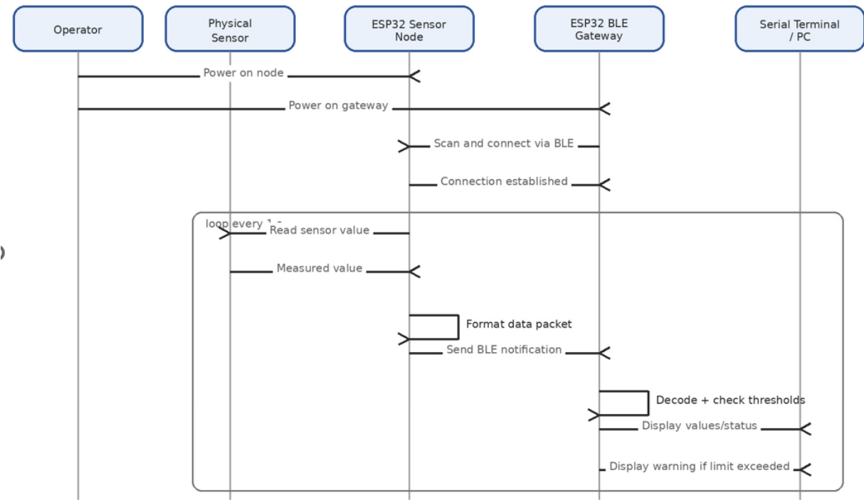
Fig. 4. Sequence diagram for normal monitoring operation. Source: self-generated by the project team.
