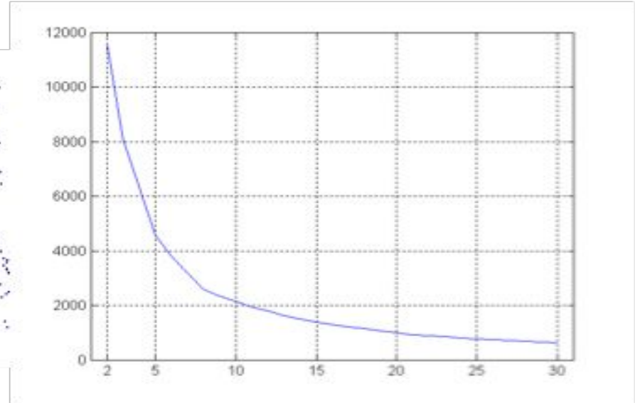
SSE of clusters found using K-means
