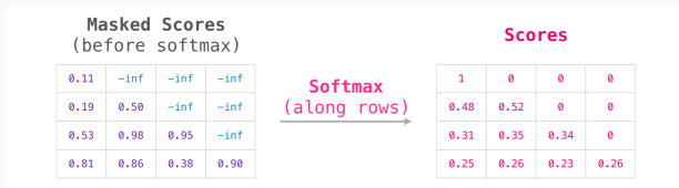
Figure 11: Finally, we compute the softmax over the masked attention scores.
