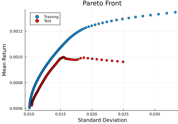
Figure 1: Train and test efficient frontier for an L2 regularised Markowitz model with a scenario-based standard deviation risk measure.
