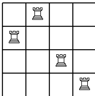
Figure 2.3: A nonattacking rook arrangement on a 4 \times 4 chessboard.
