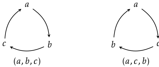
Figure 3.2: The two cycles on \{a, b, c\} . Arrows indicate the successor of each element.
