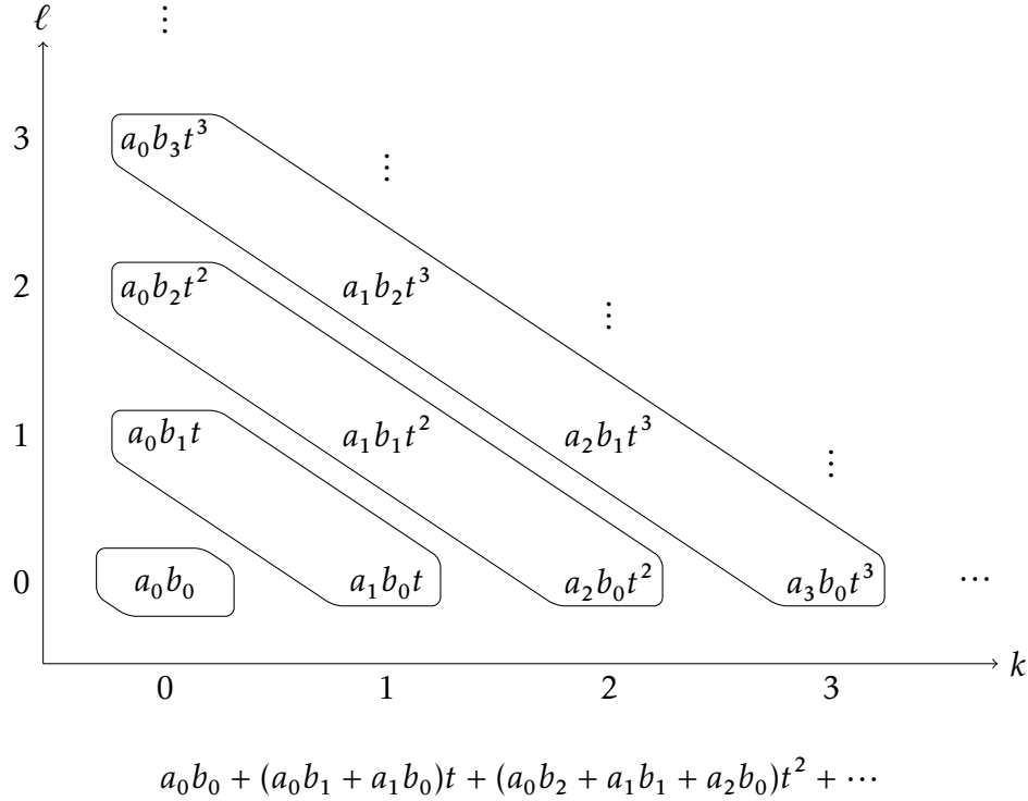
Figure 3.1: Multiplying formal power series by collecting like terms. The entry at (k, \ell) is a_k b_\ell t^{k+\ell} ; the outlined groups collect the terms of degrees 0, 1, 2, and 3.
