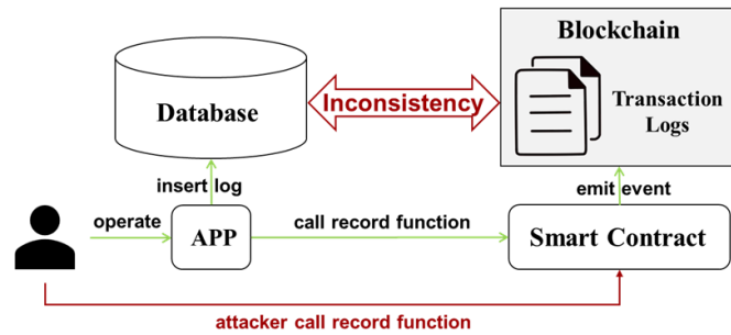
Fig. 8: The overview of Inconsistent logging apps.
