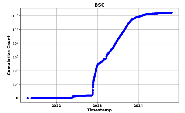
(a) BSC
