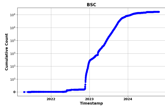
(a) BSC
