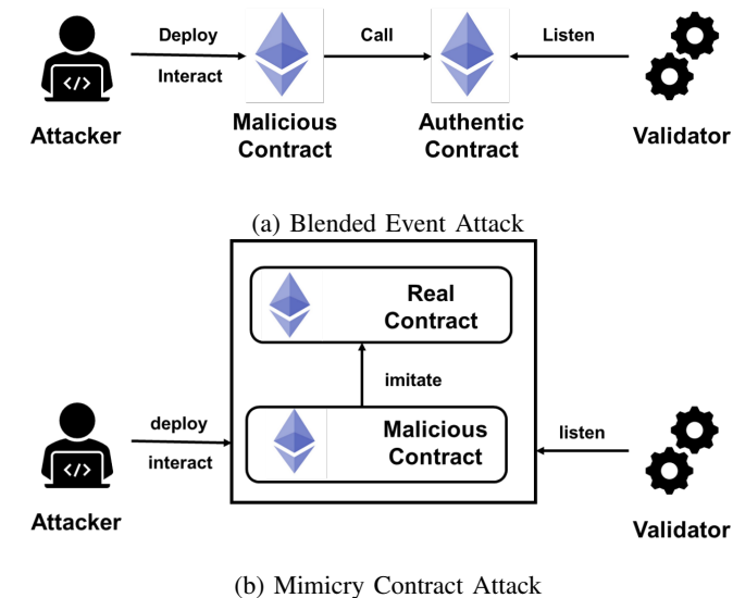
Fig. 9: Two type of Contract imitation
