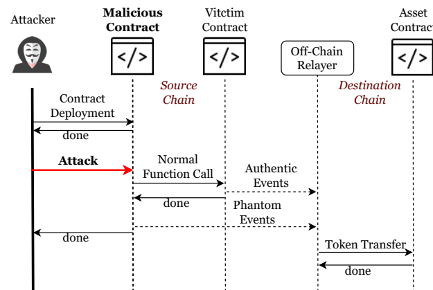
Fig. 3: Attack sequence of pNetwork Hack.
