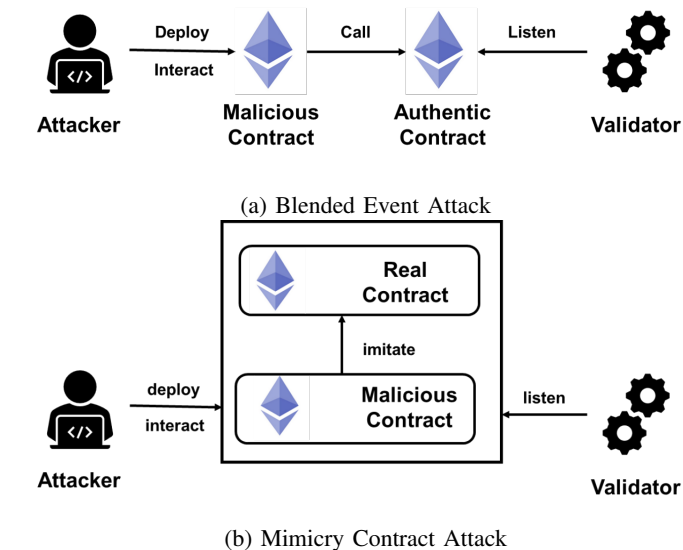
Fig. 9: Two type of Contract imitation
