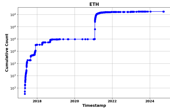
(b) ETH
