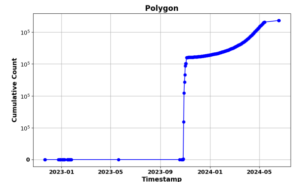
(c) Polygon
