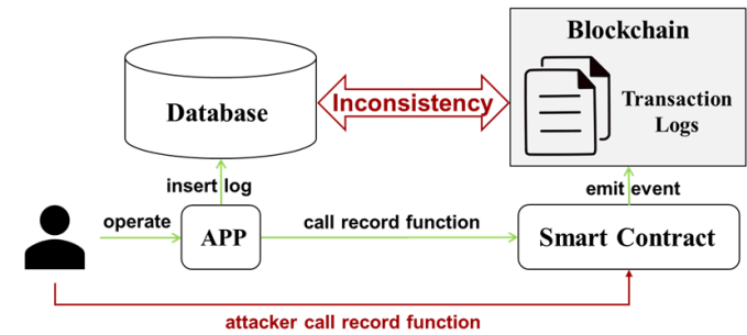
Fig. 8: The overview of Inconsistent logging apps.
