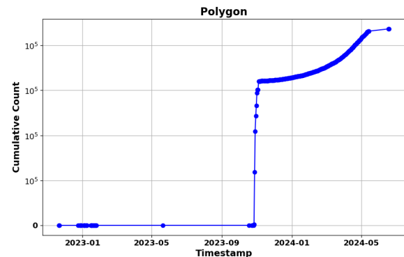
(c) Polygon
