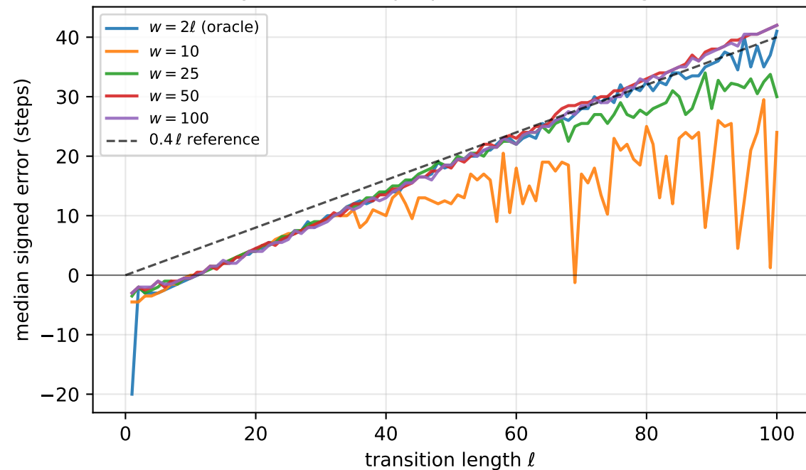
Change points fall inside the ramp, by an amount proportional to its length
