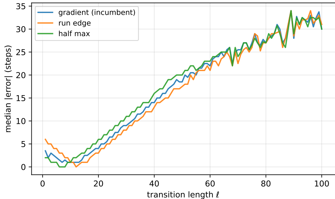
All three extraction rules share the bias ( w = 25 )
