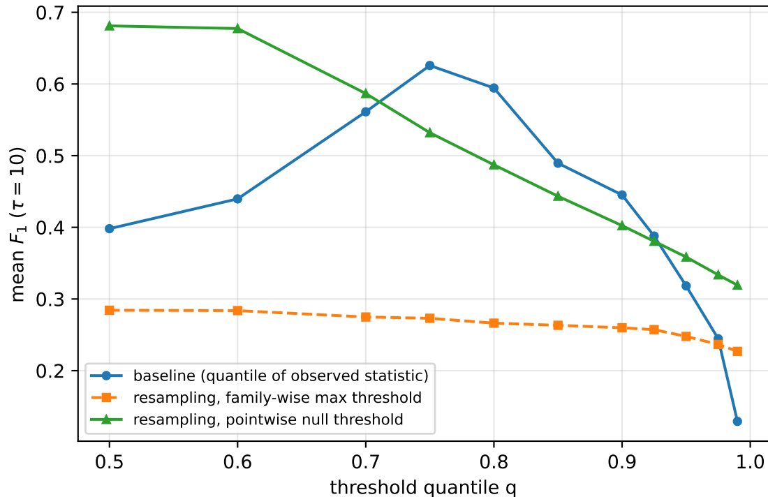
Detection quality vs. threshold quantile q
