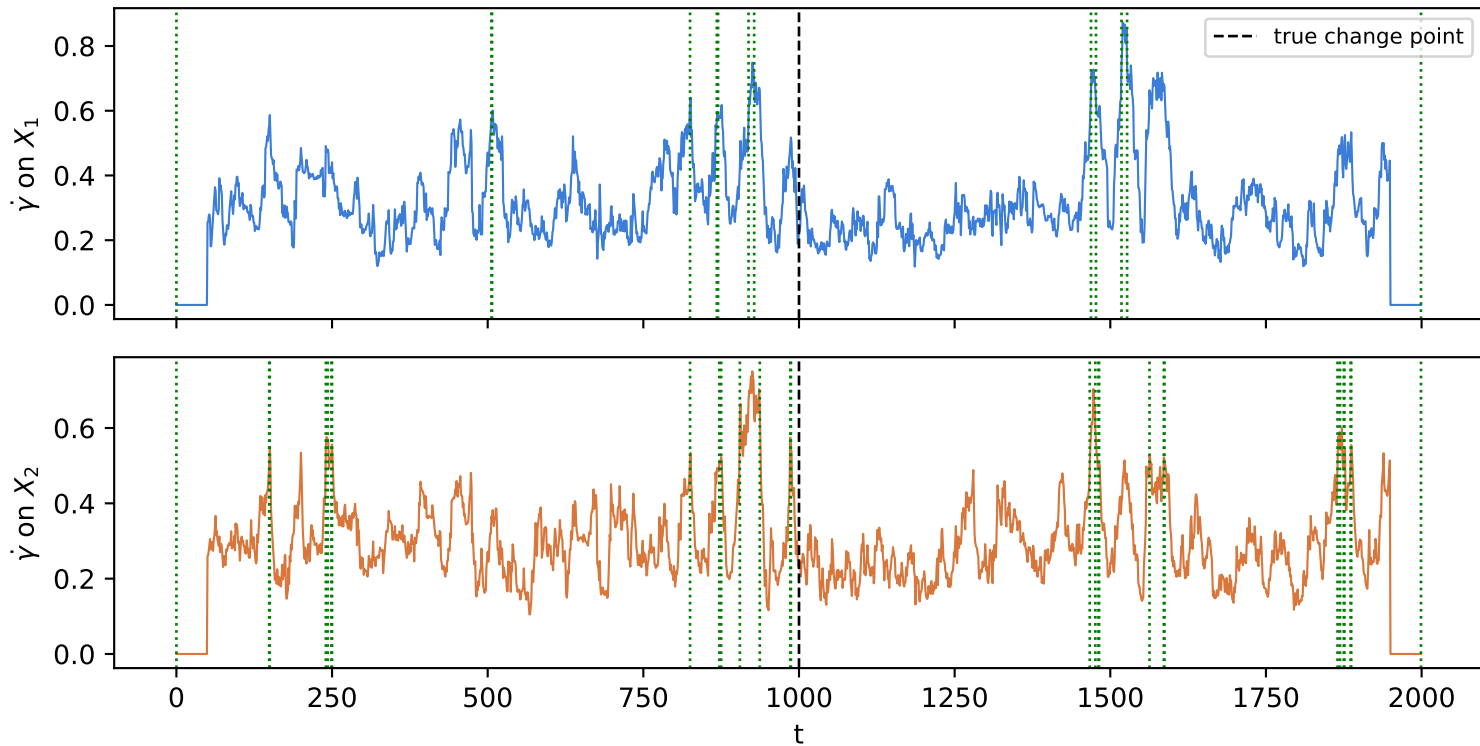
Method's own statistic (green = detected CP): no response at t^*
