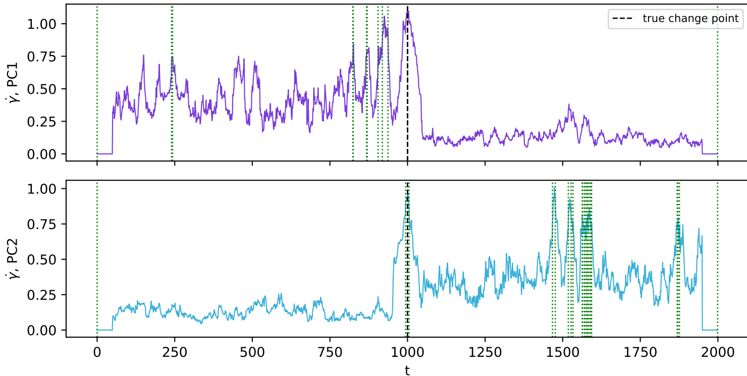
Existing 1D method run componentwise on pooled-PCA axes
