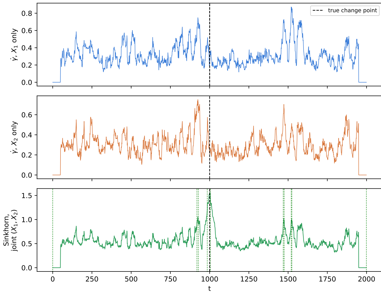
Entropic OT on the joint sample recovers t^* ; either marginal alone cannot
