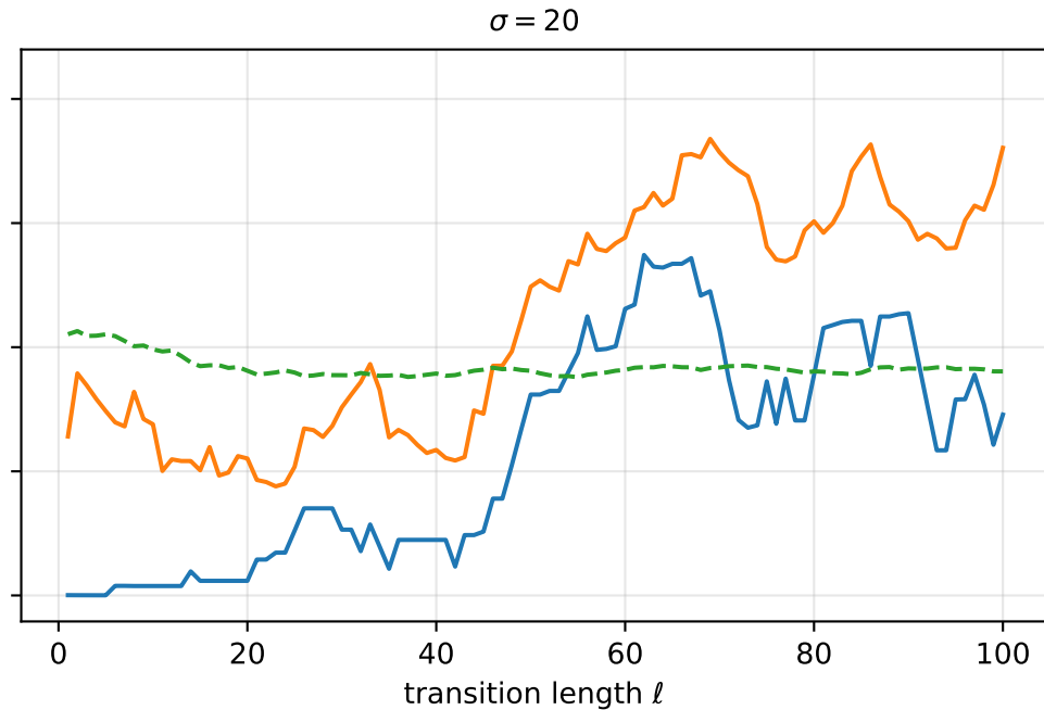
Distributional error of recovered cluster laws (lower is better)
