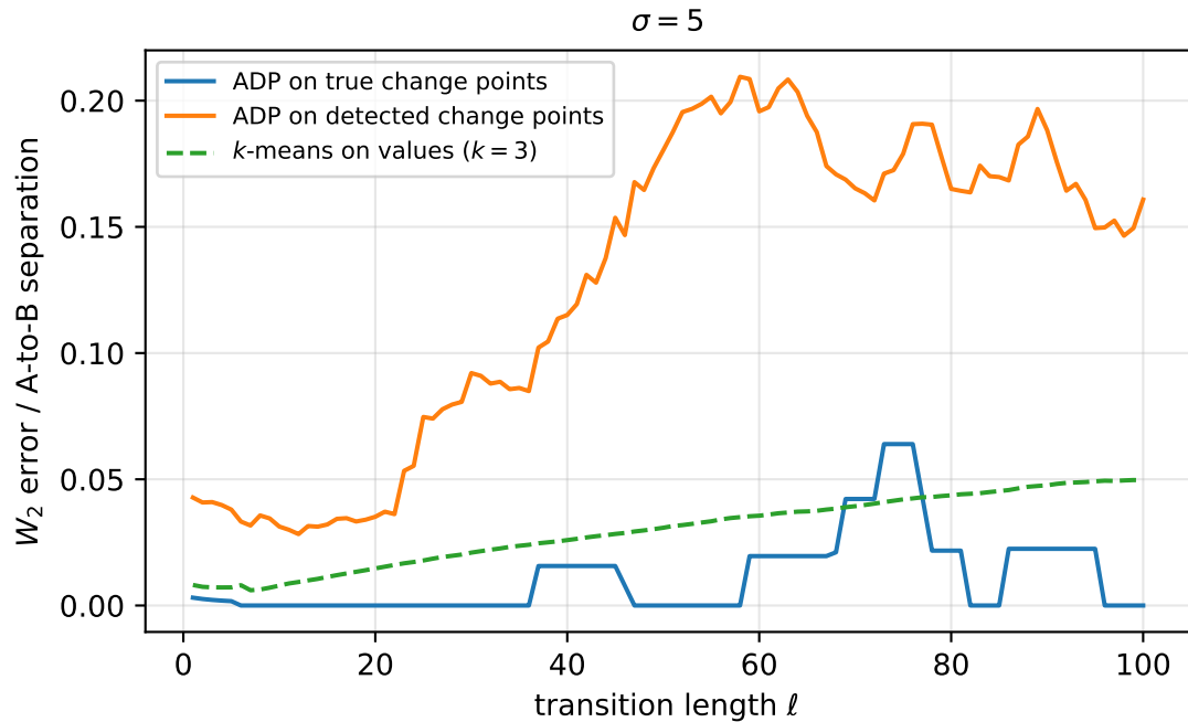
Distributional error of recovered cluster laws (lower is better)
