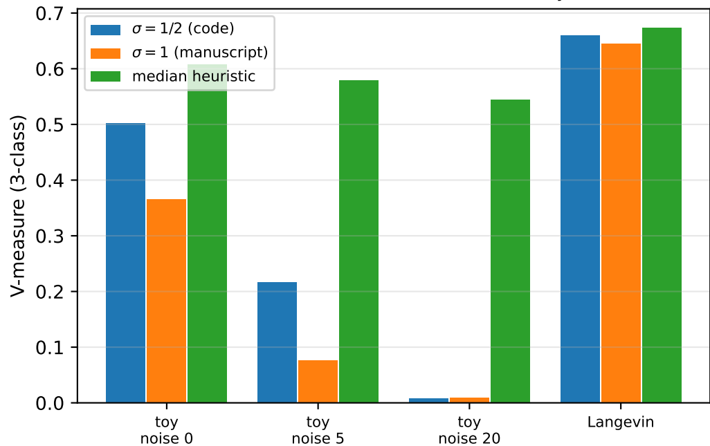
A scale-free \sigma removes the sensitivity
