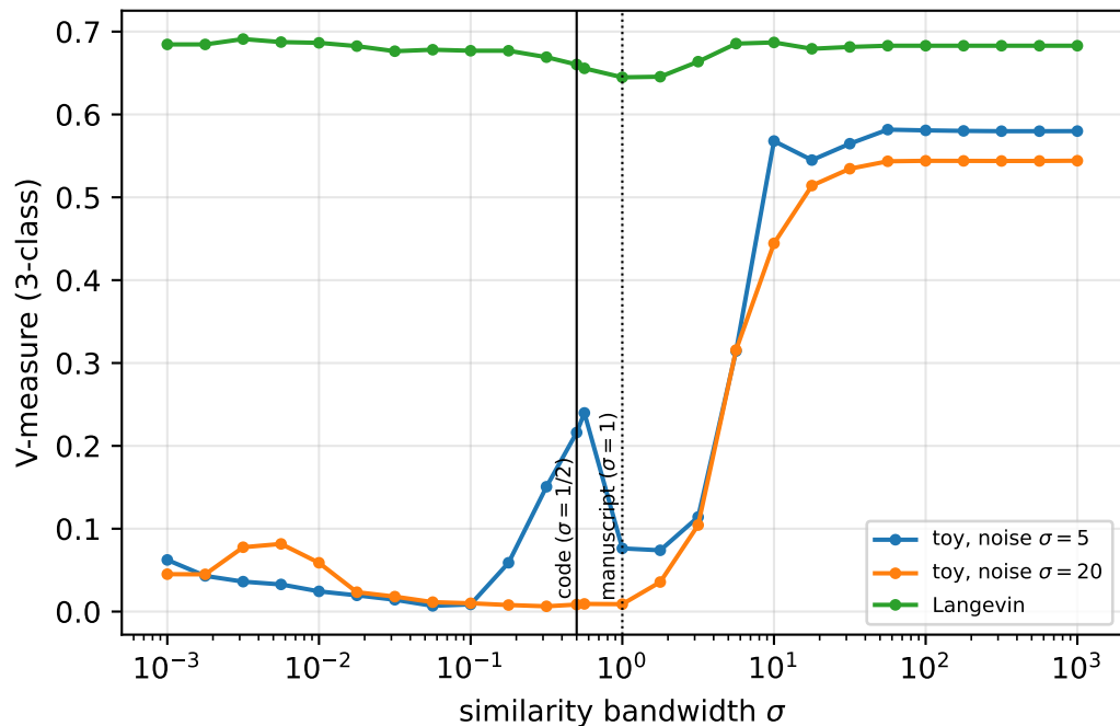
Quality vs \sigma (spectral, K = 3 )
