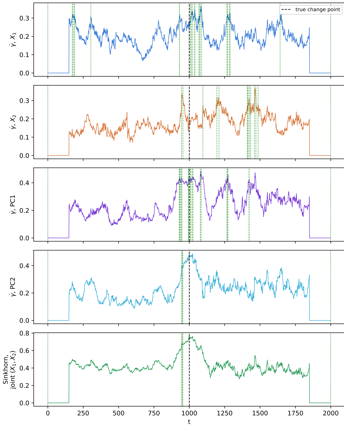
Marginals and PCA are structurally blind; Sinkhorn on the joint sample is not
