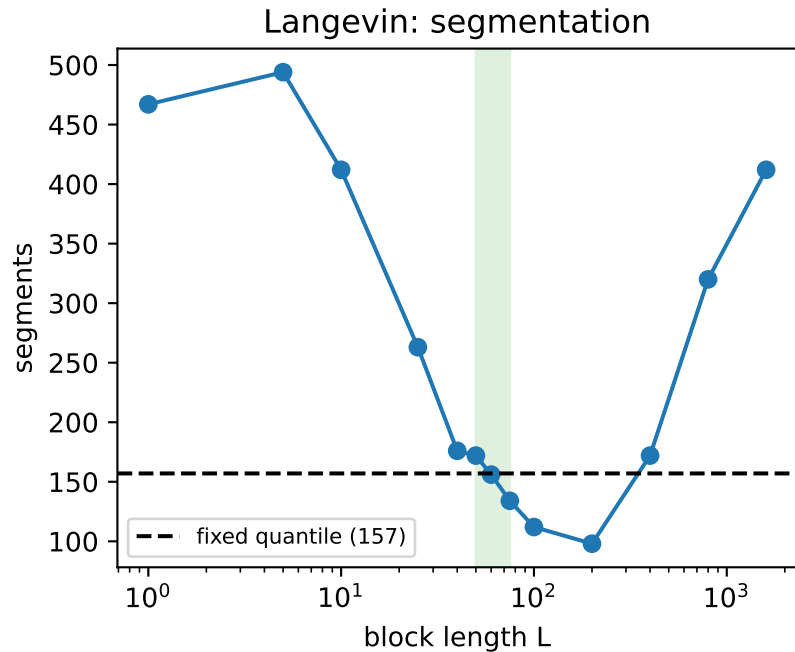
Block-permutation null vs. block length—generated by `analyze_block_permutation_null.py`
