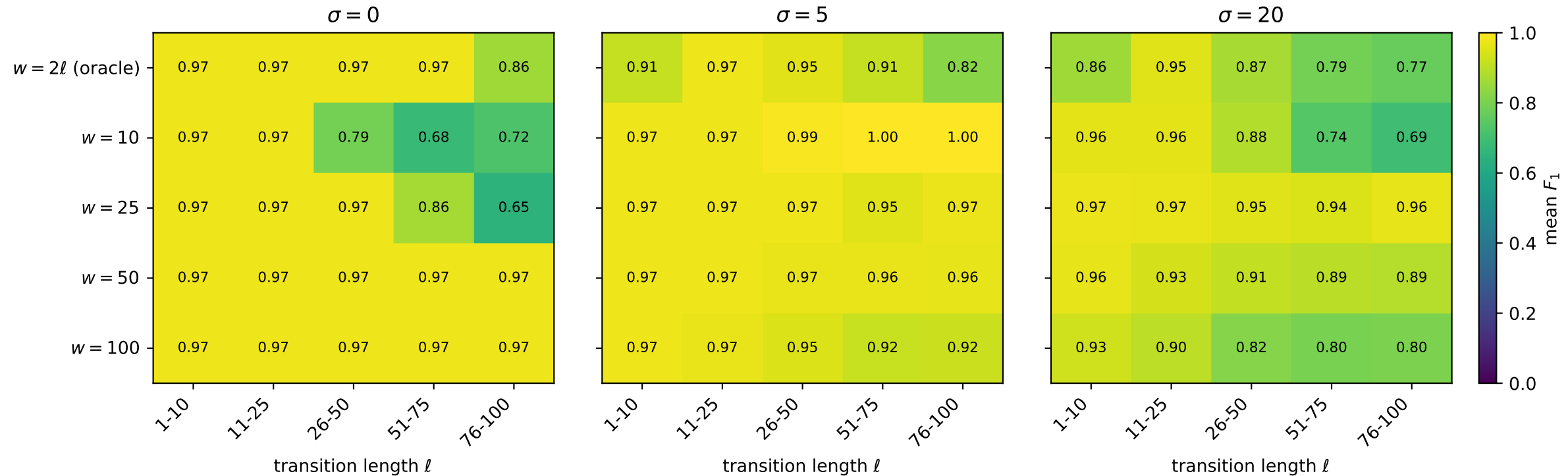
Choice of window w across noise and transition length
