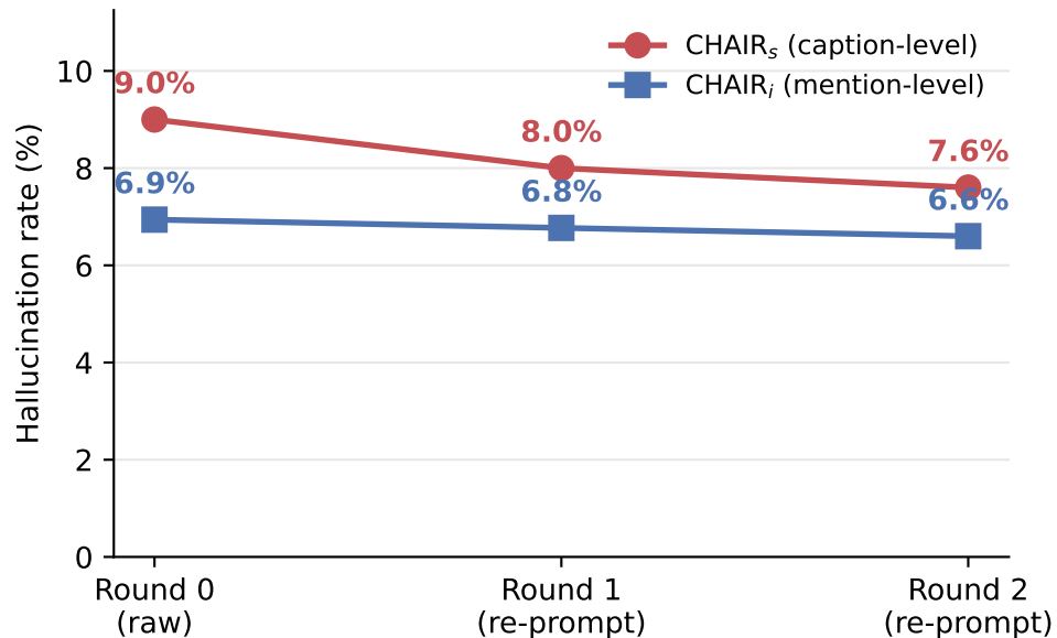
(a) Hallucination rate per round
