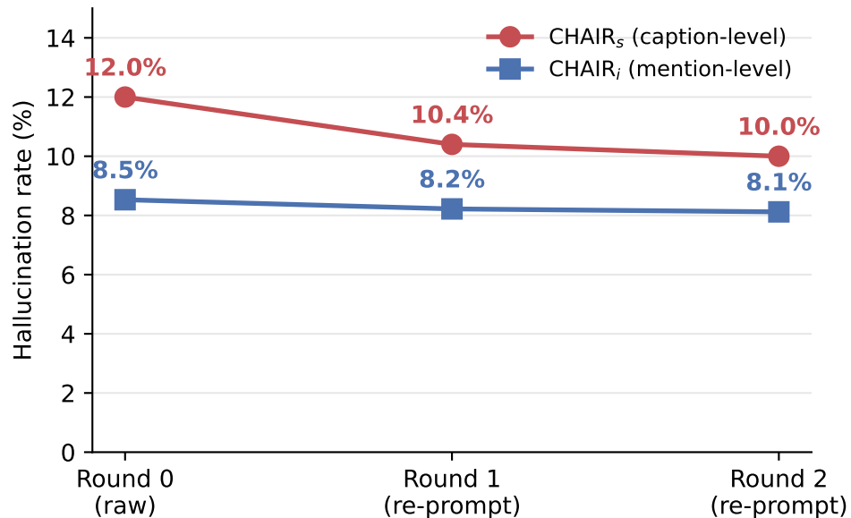
(a) Hallucination rate per round
