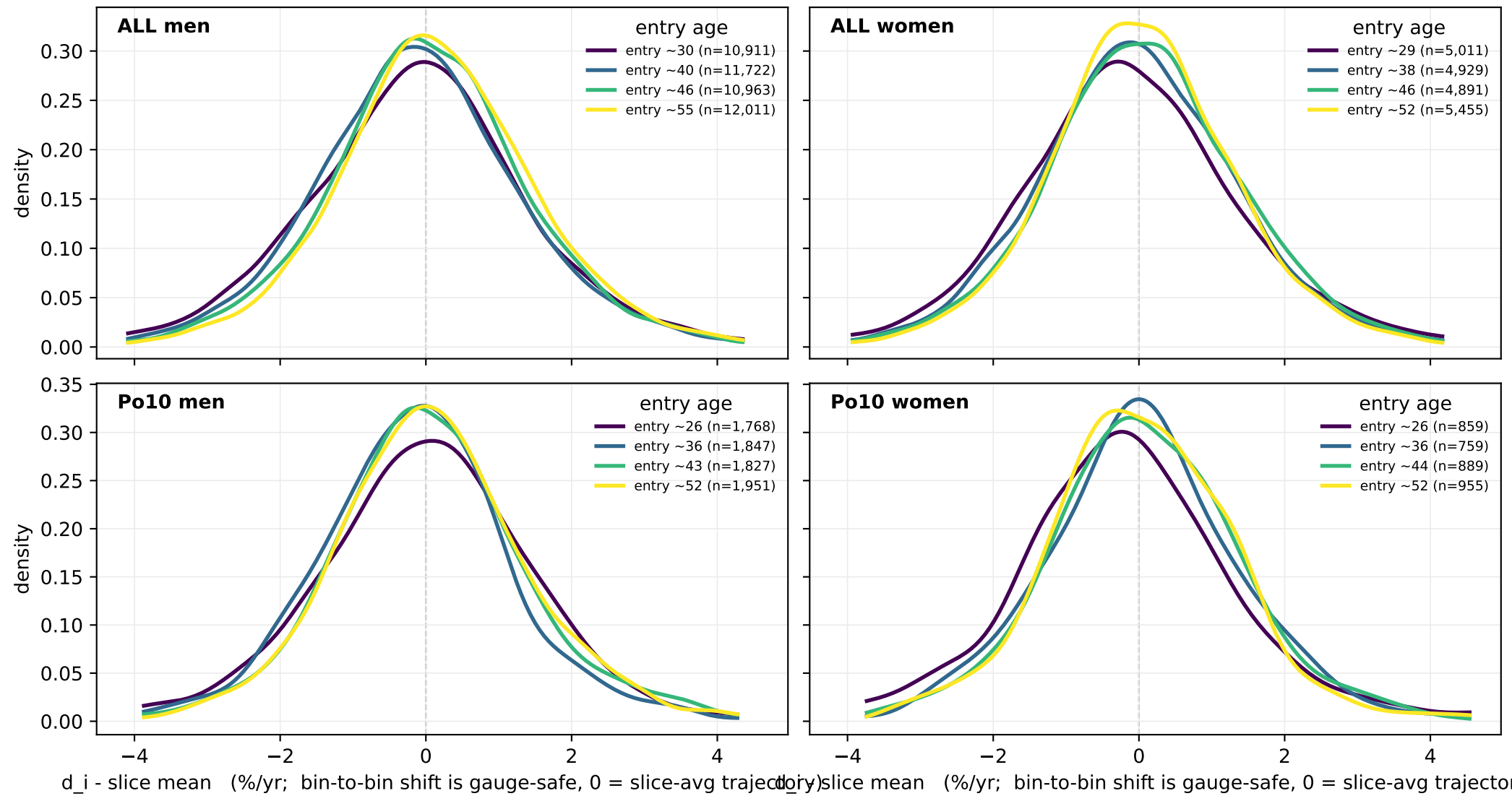
Individual career-drift d_i by entry age (full nu8, mrc2, n_i \geq 5 ; centered on slice mean)
