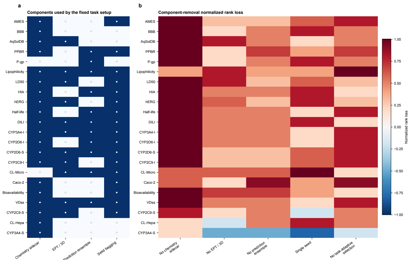
Supplementary Figure S1: Task-wise component usage and scale-free component-removal effects. a , Component map for the 22 fixed TDC ADMET task configurations. Filled circles indicate components used in the final configuration; open circles indicate components not used. b , Within-task normalized rank loss after removing each component class. Positive values indicate a worse within-task rank than the corrected full configuration, zero indicates a tie and negative values indicate an improved rank after restriction. Exact task-level scores, ranks and stability statistics are provided in Supplementary Table S23. Task labels use abbreviated dataset codes; full endpoint names are listed in Supplementary Table S1. Alt text: A two-panel matrix and heatmap show which chemistry, geometry, ensemble and seed-bagging components each of 22 tasks uses and the scale-free normalized rank loss after each component restriction.
