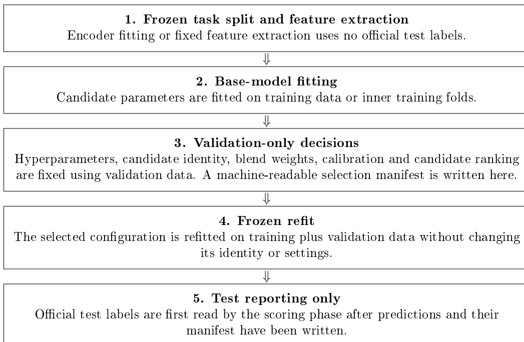
Supplementary Figure S2: Leakage-controlled development and evaluation protocol. The test split can be featurized without labels for final prediction, but its labels are inaccessible to selection and refitting code. Family-transfer candidates additionally remove source molecules matching target validation or test identities during selection and target test identities during final refitting. Alt text: Five vertically ordered boxes separate frozen splitting and feature extraction, base-model fitting, validation-only decisions, frozen train-plus-validation refitting and final test-only scoring.
