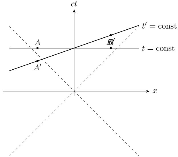
Figure 5.3: Two different simultaneity slices for observers in relative motion.
