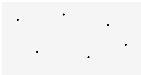
a Euclidean plane with no chosen coordinates
