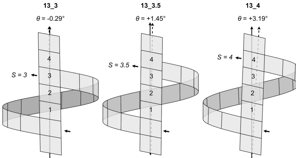
Theoretical protofilament skew angles corresponding to GDP-BeF 3 - microtubules, with a tubulin spacing ( a ) of 40.6 Å, and a rise ( r ) of 9.63 Å.
