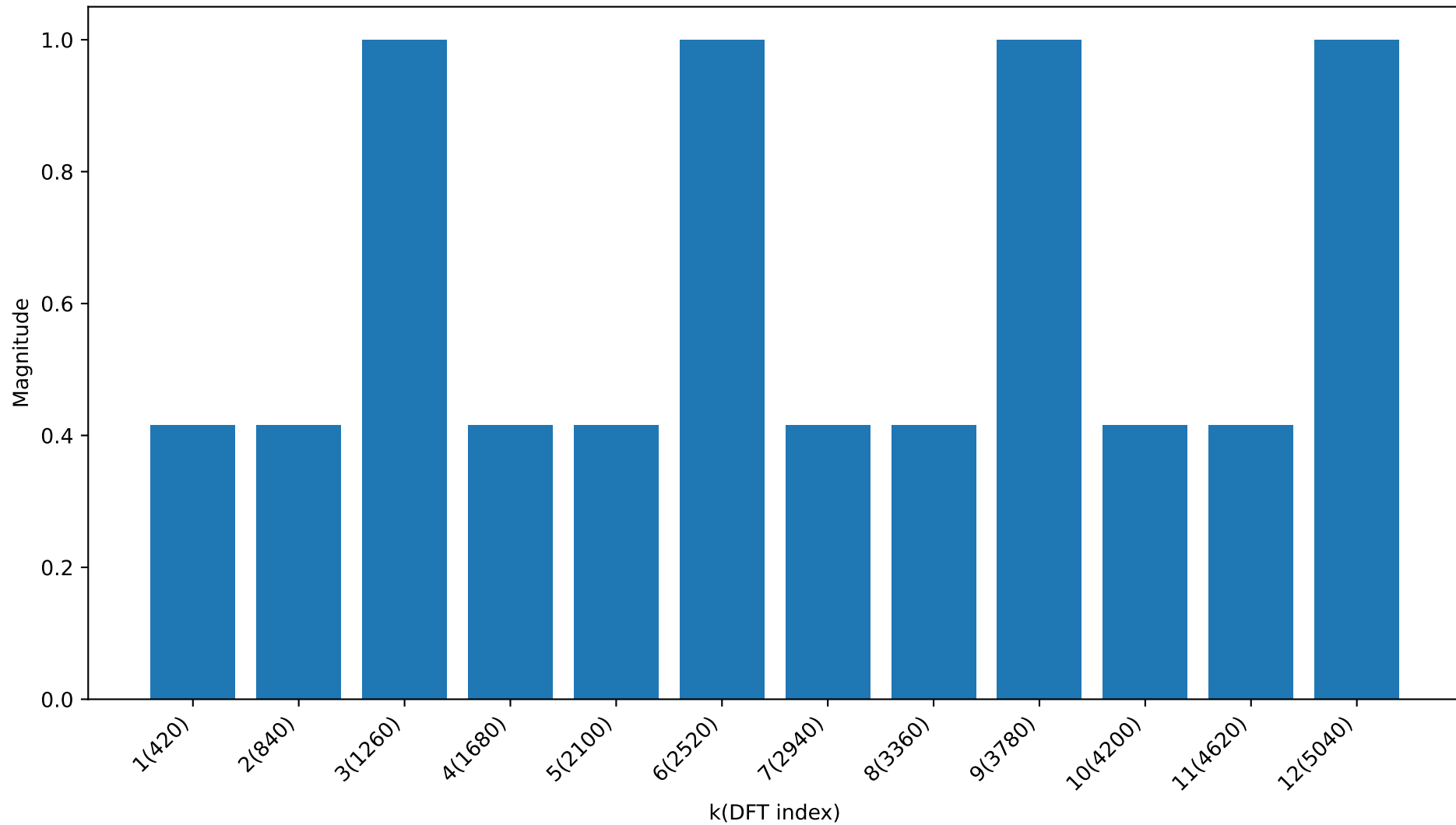
DFT Mag Redux for Meter: 6/8
