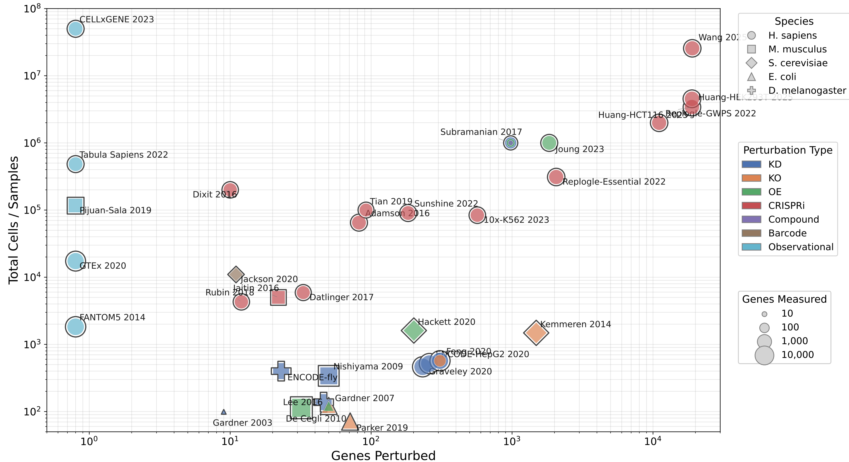
Datasets for GRN Inference (size = genes measured; shape = species; fill = perturbation type)
