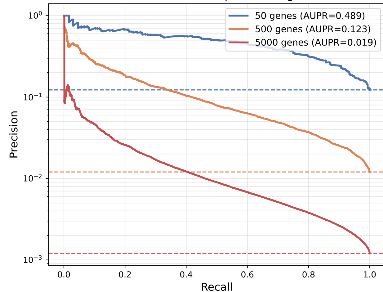
E. Subsampling inflates a poor AUPR (all sizes)
