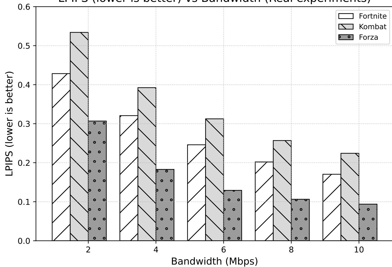
LPIPS (lower is better) vs Bandwidth (Real experiments)
