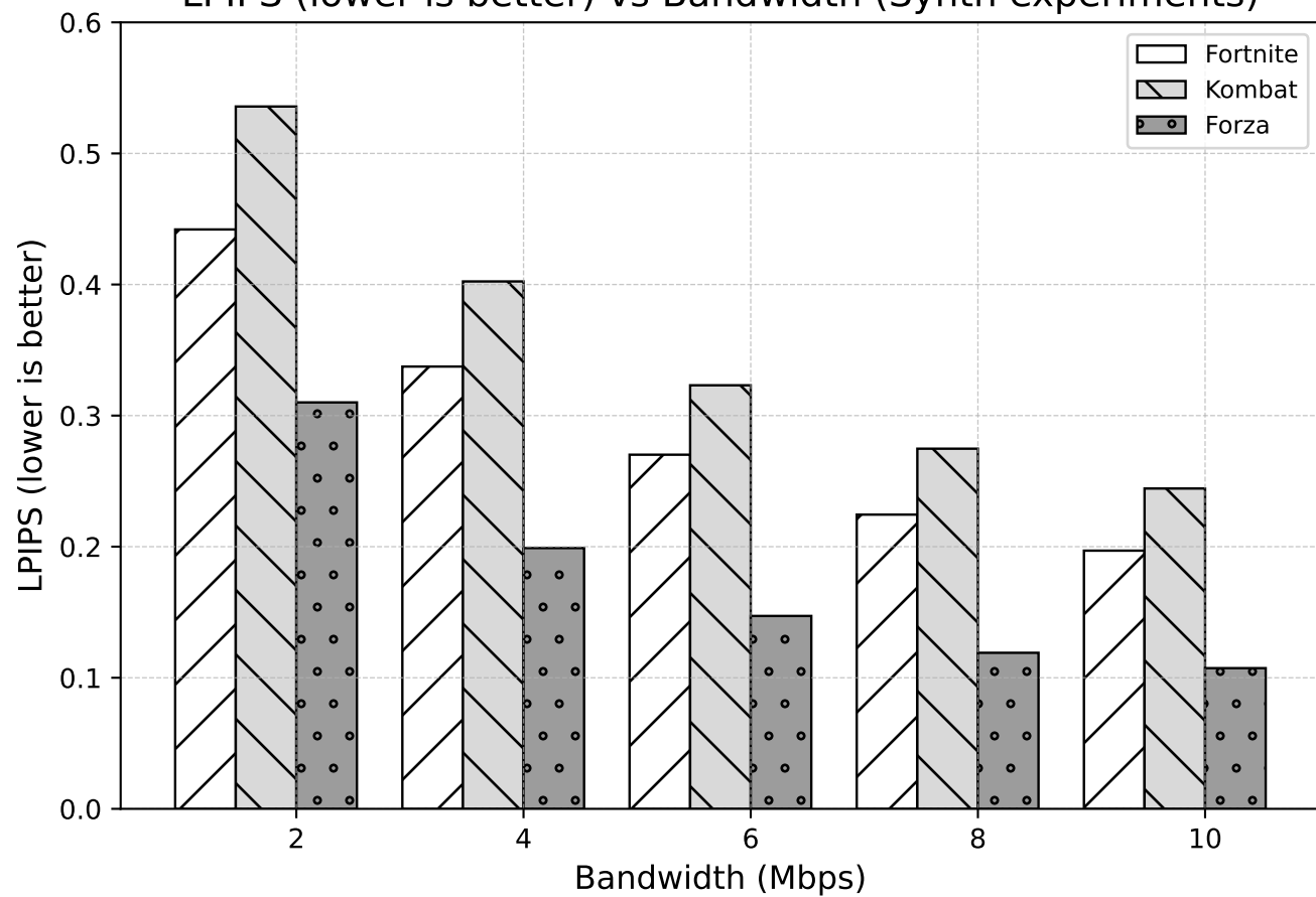
LPIPS (lower is better) vs Bandwidth (Synth experiments)
