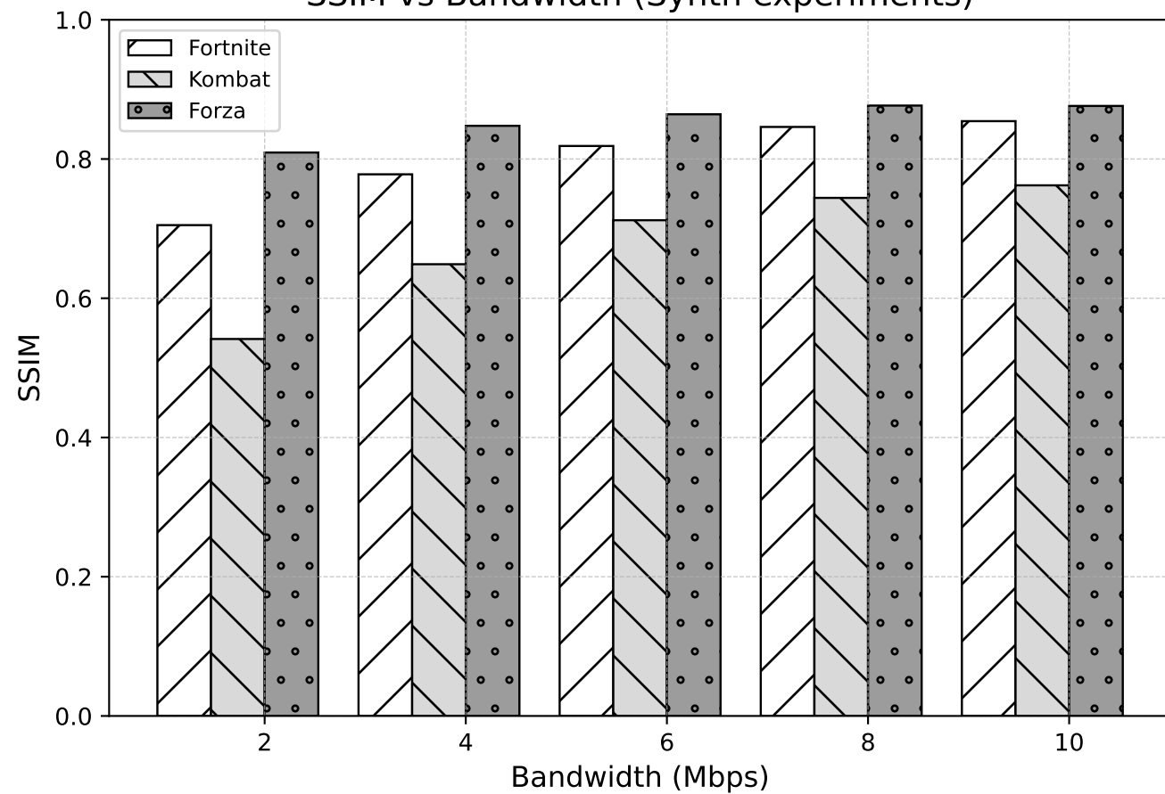
SSIM vs Bandwidth (Synth experiments)
