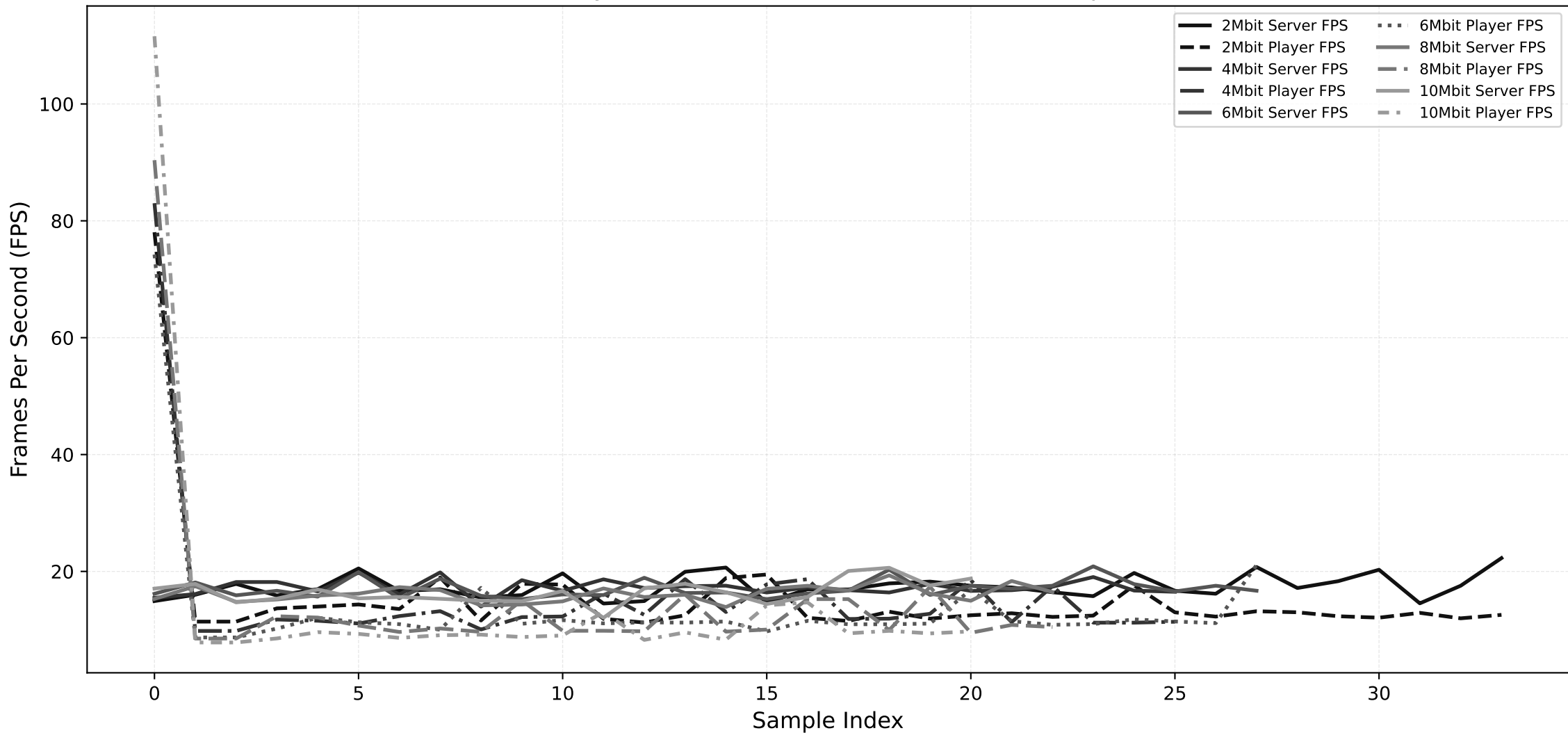
Server vs Player FPS over time for Fortnite (Real experiments)
