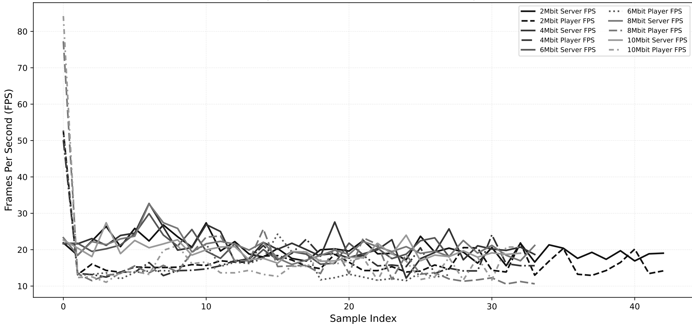
Server vs Player FPS over time for Forza (Real experiments)
