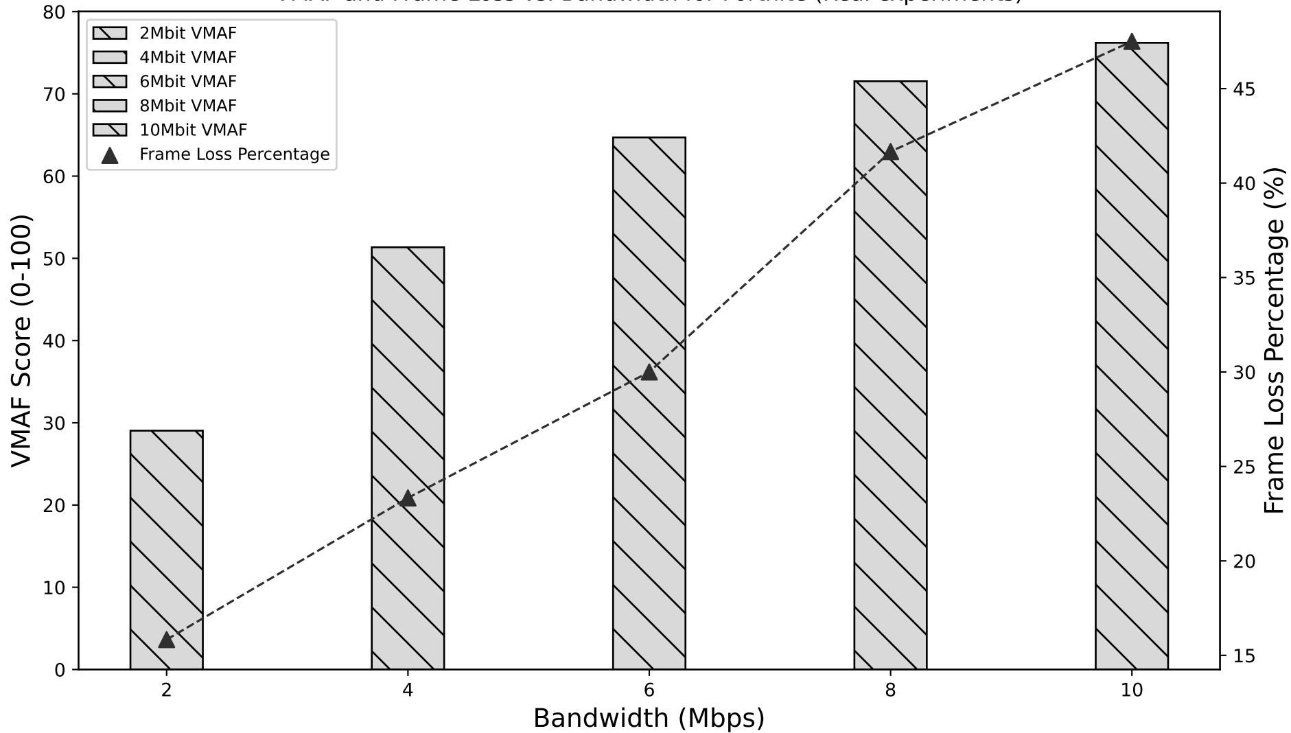
VMAF and Frame Loss vs. Bandwidth for Fortnite (Real experiments)
