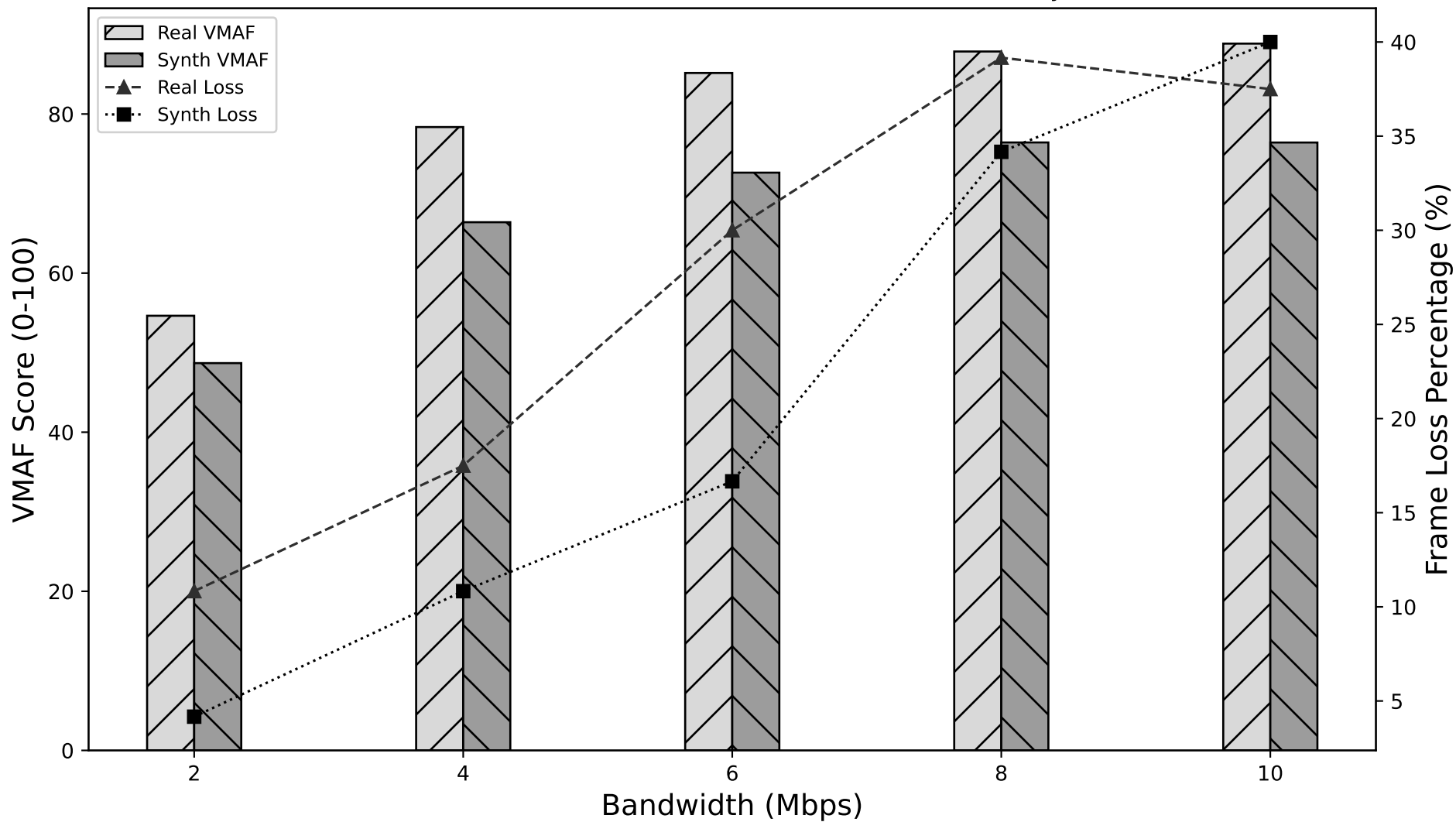
VMAF and Frame Loss vs. Bandwidth for Forza (Real vs Synth)
