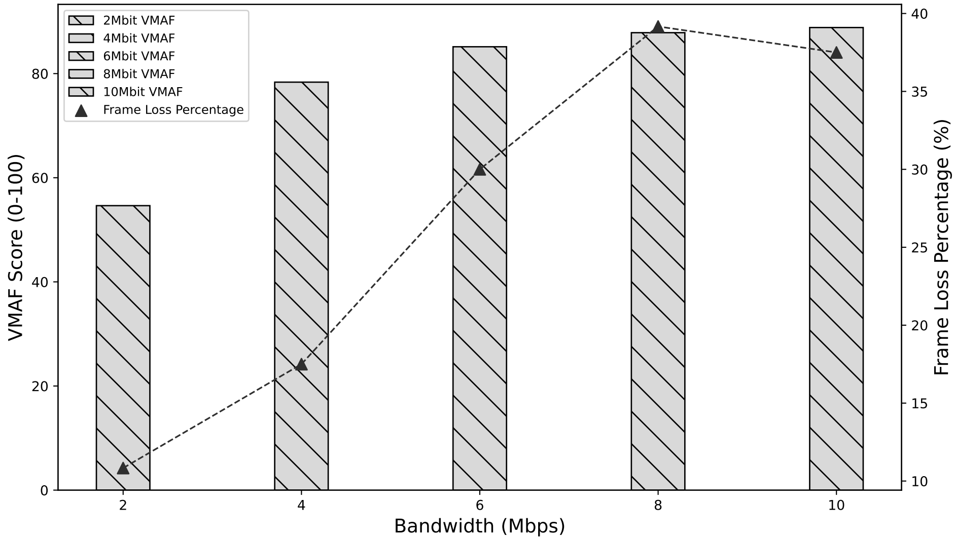
VMAF and Frame Loss vs. Bandwidth for Forza (Real experiments)
