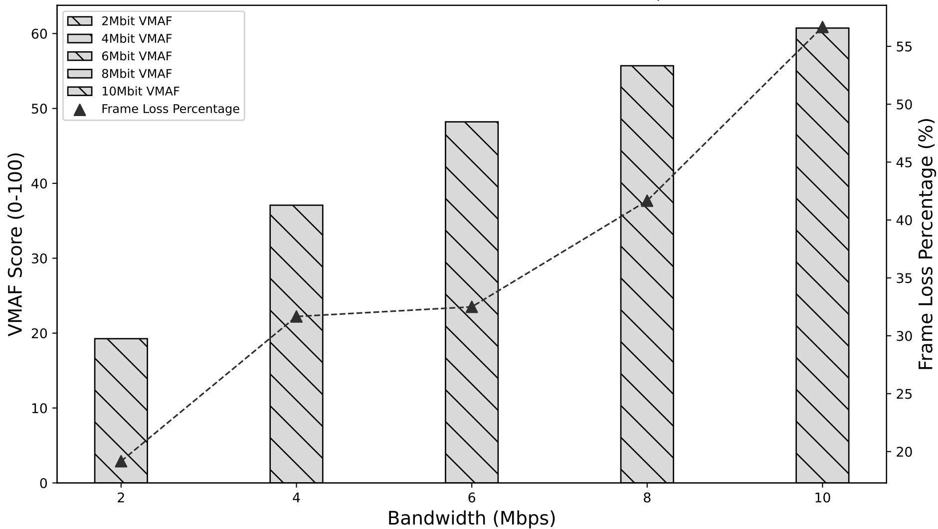
VMAF and Frame Loss vs. Bandwidth for Kombat (Real experiments)
