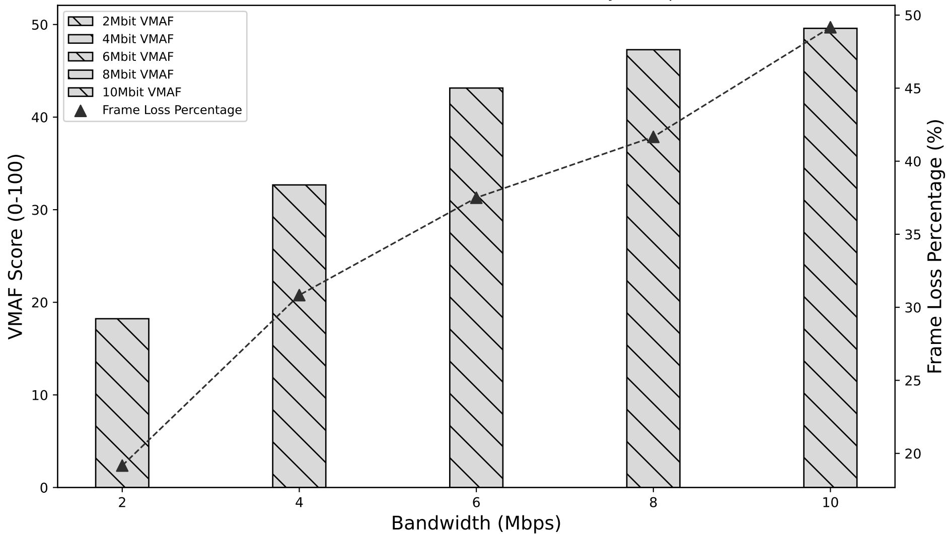
VMAF and Frame Loss vs. Bandwidth for Kombat (Synth experiments)
