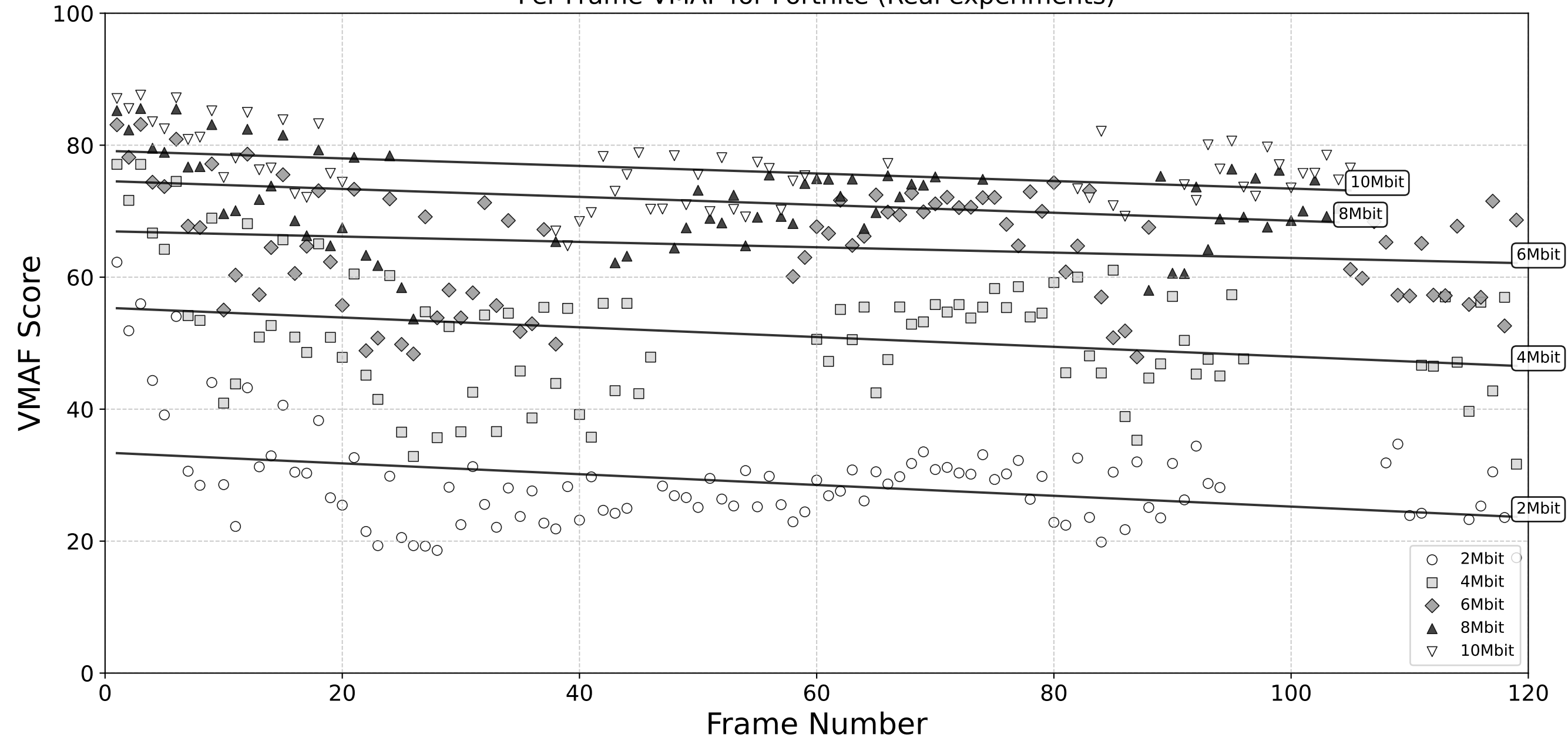
Per-Frame VMAF for Fortnite (Real experiments)
