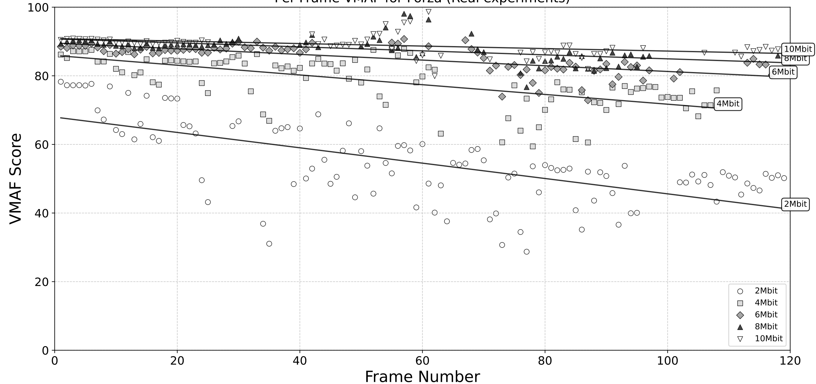
Per-Frame VMAF for Forza (Real experiments)
